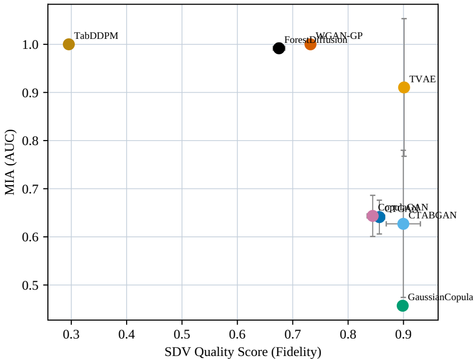
Mushroom: SDV Quality Score (Fidelity) vs MIA (AUC)
